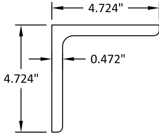
7 FIN ROOT LOW PROFILE
