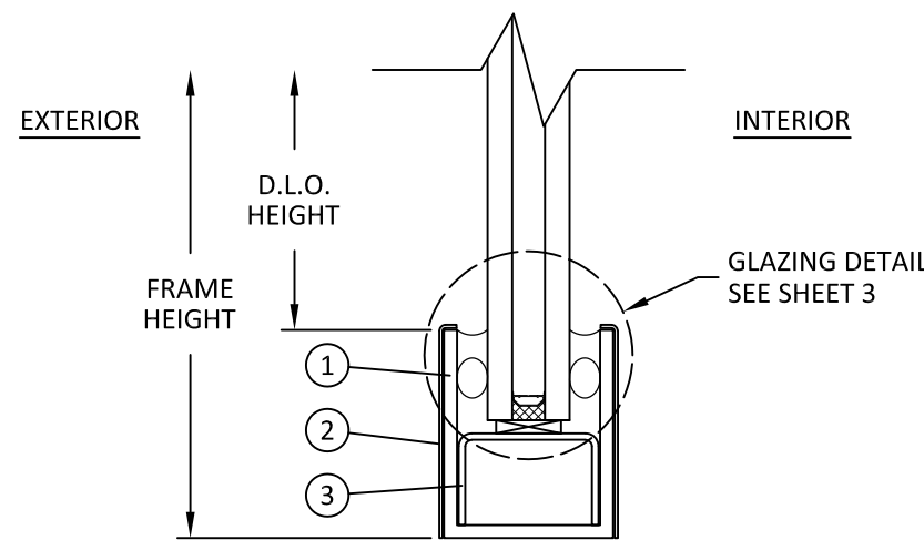
B 4 VERTICAL SECTION SILL
