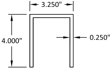
1 GLAZING CHANNEL
