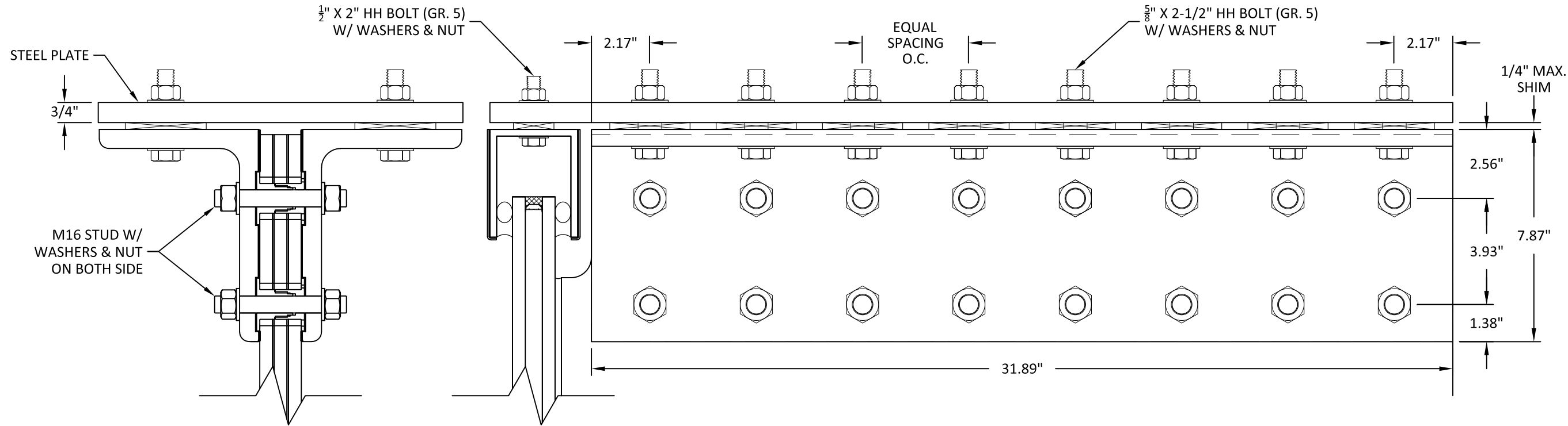
H 6 INSTALLATION DETAILS TALL WALL HEAD
