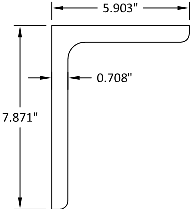
6 FIN ROOT TALL PROFILE
