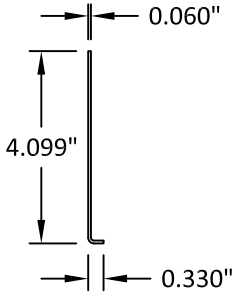
2 CHANNEL CLADDING
