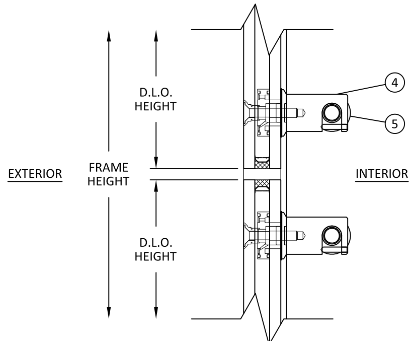
D 4 VERTICAL SECTION INTERSECTION
